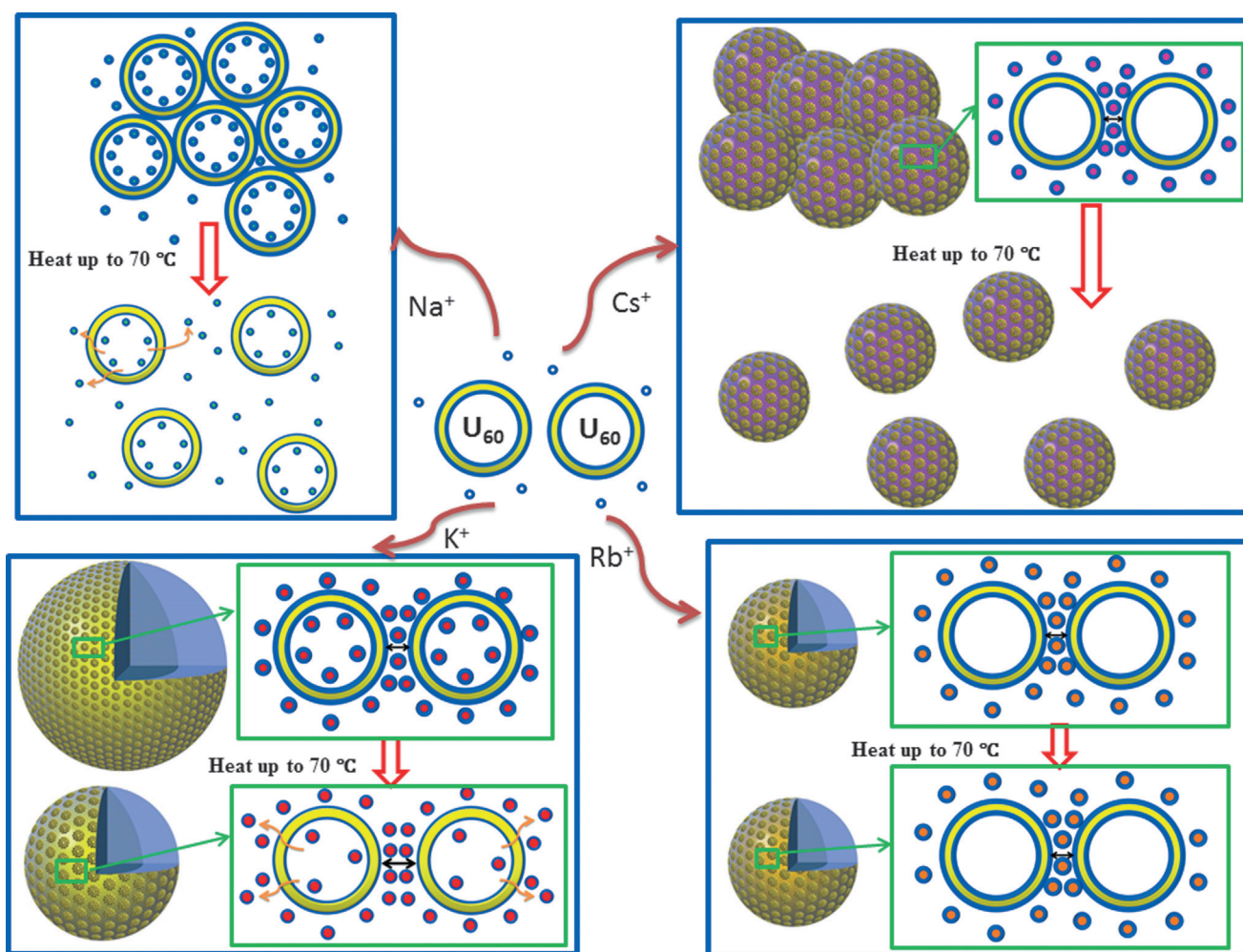
Figure 3. U_{60} clusters respond to additional alkali ions. For NaCl , U_{60} clusters tend to aggregate and precipitate at room temperature. When the temperature reaches 70 °C, U_{60} clusters are dispersed and become soluble again. For KCl , blackberries form in solution. Raising the temperature leads to a smaller blackberry size. For RbCl , blackberries form at room temperature and remain the same at 70 °C. For CsCl , U_{60} firstly self-assembles into blackberries, which gradually aggregate and precipitate. After heating the solution up to 70 °C, aggregated blackberries are separated from each other in solution. Key: U_{60} clusters (yellow circles); hydration shells (blue corona); Li^+ , K^+ , Rb^+ , and Cs^+ counterions (cyan, red, orange, and purple dots, respectively).
